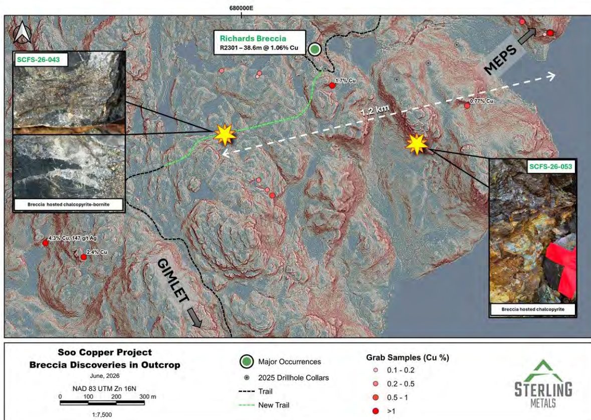
Figure 6. New Outcropping Areas of Interest seen in Parallel Structure to MEPS Discovery
